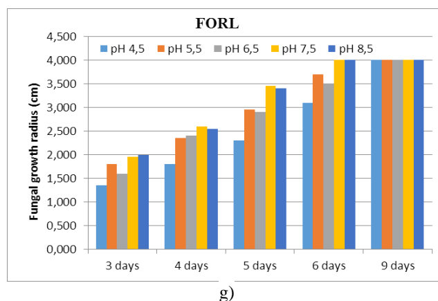
Fig. 3. Growth dynamics of the fungal strains on PDA with different pH values: a) 2TChV2 strain; b) TCh+BioV2; c) 6TChV6; d) 8 Fusarium sp.; e) 9TCh+BioV2; f) Juhwangmi P10; g) FORL.
